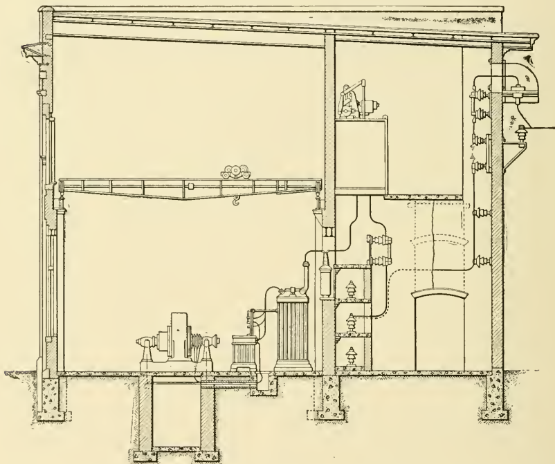
Fig. 167. Sectional Elevation of Substation for West Shore Railroad
